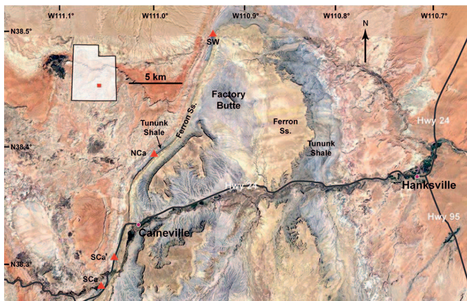
FIG. 4.—Map of the Tununk Shale outcrop belts near Hanksville. Red triangles indicate locations of three stratigraphic sections measured in this study (SW, Salt Wash; NCa, North Carneville; SCa, South Carneville). The section measured at SCa is a composite section consisting of two segments (SCa and SCa').
