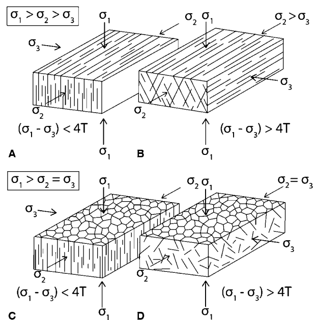
Fig. 31. The impact of the intermediate principal stress ( \sigma_2 ) on the strike direction of extensional and shear fractures. Extensional fractures form when the differential stress ( \sigma_1 - \sigma_3 ) < four times the tensile strength ( T ) and shear fractures when it is > 4T . In (A) and (B), \sigma_2 > \sigma_3 and the strike orientations of the resulting fractures are consistent and regular. In (C) and (D), \sigma_2 = \sigma_3 and the fracture strike directions are random, resulting in polygonal arrays. Note that Fig. 31C is the stress regime proposed for the Sheepbed mudstone during the evolution of the vein system it contains. From Cosgrove & Hudson (2016).
