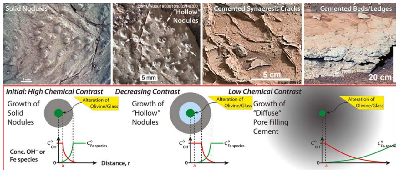
Fig. 20. Envisioned progression (from left to right) of early diagenetic features as olivine/glass alteration reaction dissipates through the pore space. The top row shows representative images of the various diagenetic features that form as a consequence of this process. The bottom row shows a model of centrifugal and counter diffusion of two reactive species at various levels of chemical contrast with the surrounding pore waters, how the saturation index may be exceeded at the centre (solid nodules) or at some distance (hollow nodule, cement shell) from the reacting grain, and how at lowest contrast cementation of sphaeresis cracks (raised ridges) and the matrix (cemented ledges) occurs. Based on a two-dimensional model developed by Helfferich & Katchalsky (1970) which was developed into a 3D model by Raiswell et al. (1993). Images from left to right: MAHLI image 0276MH0002650000103019R00; MAHLI image 0291MH0001900010103314C00; Mastcam Right image 0164MR0008850060201595E01; Mastcam Left image 0298ML0012440030106396E01. MAHLI, Mars Hand Lens Imager.
