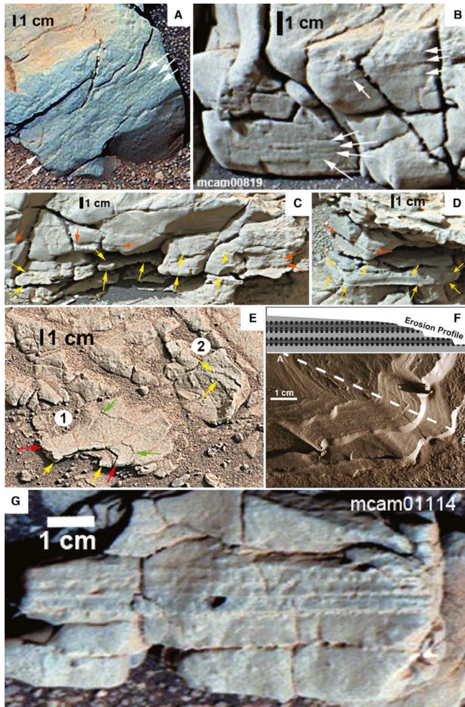
Fig. 5. (A) Side view of a piece of mudstone polygon in Sheepbed unit 1. Arrows point to faintly developed internal parallel layers at the centimetre-scale. Mastcam Right image 0297ML0012420030106392E01. (B), (C) and (D), examples of millimetre to centimetre-scale internal layering in Sheepbed unit 2. White arrows point to largely parallel laminae, red arrows mark laminae that can only be traced for short distances, and yellow arrows mark thin beds. Thin bed in (D) has a more resistant base, might be graded. (B) Mastcam Right image 0138MR0008190650201079E01, (C) Mastcam Right image, 0138MR0008190620201076E01, (D) Mastcam Right image 0138MR0008190610201075E01. (E) A bed surface with traces of resistant laminae (locations 1 and 2, arrows) that look like they might have been 'etched out' by aeolian abrasion. Mastcam Right image 0147MR0008350010201199C00. (F) Lower portion shows terrestrial shale where experimental aeolian abrasion accentuated differences in layer hardness that look very similar to what is seen in (E). Upper portion shows step-wise erosion of shale laminae in cross-section along white dashed line A–B. Dotted black lines mark thin sub-millimetre silt laminae that are better cemented. (G) Millimetre-scale parallel laminae in a piece of Sheepbed float. Mastcam Right image 0234MR0011140180203149E01.
