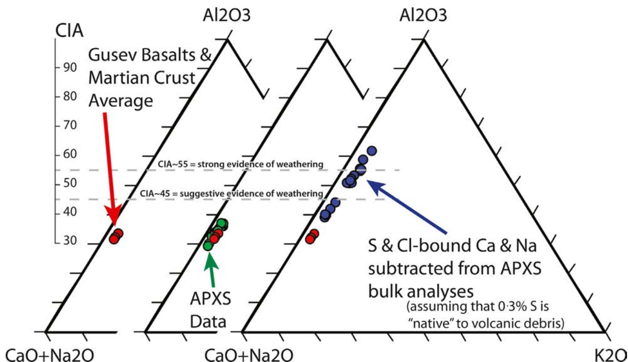
Fig. 8. Plots of potential source rocks and Sheepbed APXS data (from McLennan et al. , 2014) with regard to the molar proportions of the elements that constitute the chemical index of alteration (CIA; Nesbitt & Young, 1982). The left plot shows the position of the Martian crustal average (Taylor & McLennan, 2009) and basalts from Gusev crater on Mars (McSween et al. , 2006a,b). The middle plot shows in addition the positions of APXS data as reported by McLennan et al. (2014), and the tight clustering of these analyses near the crustal and basalt compositions. The right plot shows APXS analyses from the Sheepbed member that have been ‘corrected’ for that amount of Ca and Na that are probably bound to sulphur and chlorine. The whole-rock APXS analyses plotted here were reported by McLennan et al. (2014), and that publication also contains information on methodology and instrumentation as well as further references. APXS, Alpha Particle X-Ray Spectrometer.
