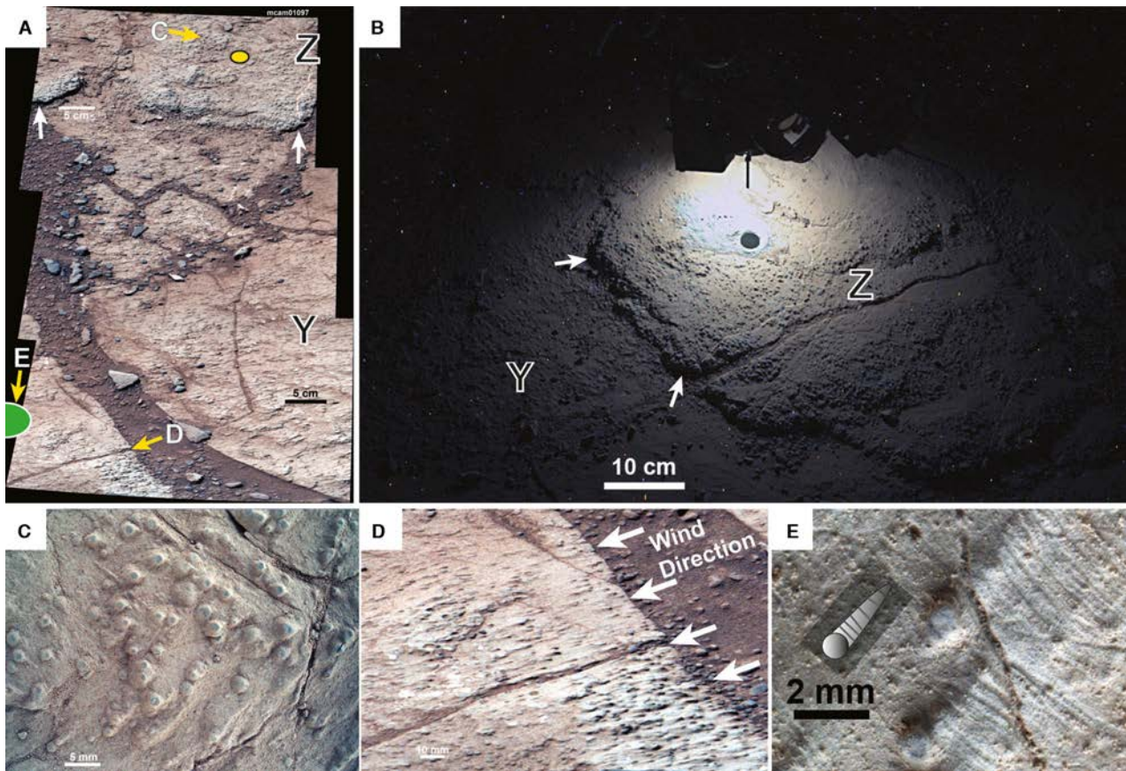
Fig. 15. (A) A Mastcam Right mosaic acquired on Sol 227 (images 0227MR0010970000202900E01, 0227MR0010970030202903E01 and 0227MR0010970060202906E01) that shows a closer view of the Cumberland drill site and its vicinity. White arrows point to a boundary between two layers, presumed to be layers Y and Z as marked in Fig. 7A. Layer Z appears more erosion resistant and differs in surface texture from layer Y. Yellow oval marks Cumberland drill hole, green oval marks Cumberland brush spot (DRT). Yellow arrows and letters 'C', 'D' and 'E' point out detail features below. (B) The rover never sleeps. Night imaging of Cumberland drill hole with MAHLI (using LED illumination), image taken by Mastcam Left (0292ML0012290010106381E01). The image brings out the contrast between layers Y and Z (contact marked by arrows). (C) Closer view of the surface of layer Z. Shows the rounded features that have been described as nodules in prior publications (Grotzinger et al. , 2014; Stack et al. , 2014). MAHLI image 0276MH0002650000103019R00. (D) Closer view of the surface of layer Y. Round features (presumed to be nodules) consistently have an elongate tail to the left. At the edge of the slab wind erosion has worn down the layer by 10 to 20 mm. Mastcam Right image 0227MR0010970060202906E01. (E) An even closer look at the surface of layer Y at the Cumberland DRT. The round nodules show no damage (scratching) from the DRT, but the wind shadow tails have been scratched by the DRT steel bristles (Fig. 1E). The inset line drawing emphasizes the observed features, scratched wind tail and scratch resistant nodule. MAHLI image 0295MH0002760000103652R00. MAHLI, Mars Hand Lens Imager.
