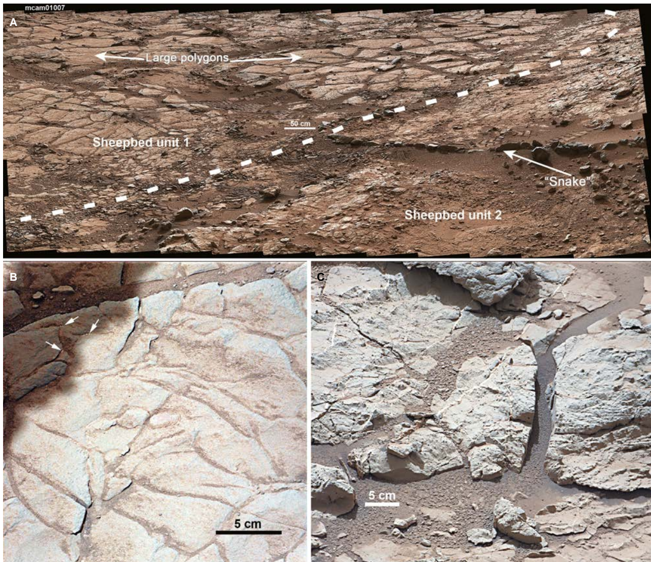
Fig. 4. (A) Dashed line separates Sheepbed unit 1 (on left, large low-amplitude convex smooth polygons) from Sheepbed unit 2 (on right, hackly weathering, smaller fragments). The cross-cutting feature named 'snake' has been interpreted as a clastic dyke of sandstone composition (Grotzinger et al. , 2014). Portion of a Mastcam Right mosaic from Sol 198 (mcam01007). (B) Closer view of smoothed polygon surface in Sheepbed unit 1. Debris filled crack near top of image. White arrows point to white crack fills of \text{CaSO}_4 (anhydrite). Mastcam Right image 0129MR0007940010200824E01. (C) Contrasting appearance of Sheepbed unit 2 with sharp edged crack margins, ragged surfaces and sub-millimetre nodules (Grotzinger et al. , 2014). Mastcam Right image 0126MR0007800000200786E01.
