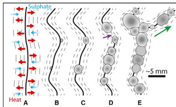
Fig. 32. Evolution of knobby veins. (A) Overpressuring due to compaction causes fractures in the consolidating mud. Warm fluids rise from depth into colder sediments with dissolved calcium sulphate and gypsum (as suggested by XRD data, and predicted by the calculation in Fig. 11) in the mud matrix. The temperature of the wall zones of fractures increases, anhydrite precipitates, and more \text{CaSO}_4 diffuses in. (B) First clusters of anhydrite begin to sprout and push into surrounding sediment. Veins may become deformed. (C) As the process continues, anhydrite clusters expand. (D) More and more anhydrite clusters form, but in some parts of the vein no anhydrite precipitates. These portions will pinch shut (purple arrow) once fluid pressure declines (see, for example, Fig. 23). (E) Initial vein may clog with anhydrite and alternative fluid routes develop (green arrow).
