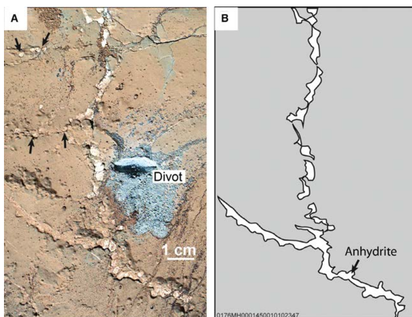
Fig. 25. (A) Image of bedding plane with drill divot scar. Bedding plane is cut by subvertical anhydrite veins. MAHLI image 0176MH0001450010102347C00. (B) Shows a sketch of the anhydrite fill. Instead of being simple filled fractures, these veins have a more complex knobbly morphology. If the anhydrite were removed, the vein walls would not fit back together. MAHLI, Mars Hand Lens Imager.
