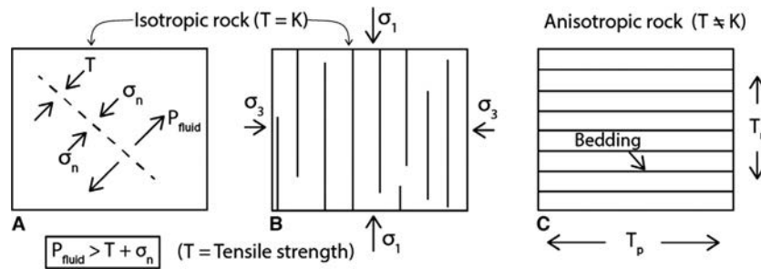
Fig. 33. (A) A block of isotropic rock and the conditions necessary to induce a hydraulic fracture parallel to the dashed line. (B) The block in (A) subjected to an overburden load ( \sigma_1 ) and an induced horizontal stress ( \sigma_3 ). Conditions for hydraulic fracturing are first met along the vertical planes normal to \sigma_3 . (C) An anisotropic (bedded) rock subjected to the same stress field as the rock in (B): T_p is the tensile strength parallel to bedding and T_n is the tensile strength normal to bedding.
