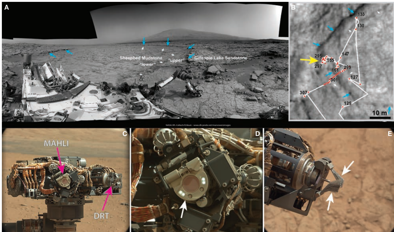
Fig. 1. (A) Black and white Navcam panorama (Sol 168, sequences ncam05794, ncam07754 and ncam12754; Sol 169 sequence ncam05794) that shows Mt. Sharp in the distance. Yellowknife Bay with the Sheepbed mudstone is left of centre, the Gillespie Lake sandstone in the centre and to the right, and the instrument turret of the rover arm is set down at the John Klein drill site. Small white arrows point to a stratigraphic boundary within the Sheepbed member that is also visible from orbit. This boundary marks in the context of this paper the contact between unit 1 and unit 2 of the Sheepbed mudstone. Blue arrows mark the erosion-resistant escarpment formed by the Gillespie Lake sandstone. (B) The path of the rover in Yellowknife Bay. Red dots and black numbers mark Sol locations. It is apparent that most time was spent in the westernmost portion (yellow arrow) on investigations of Sheepbed unit 2. Blue and white arrows mark same features as shown in (A). (C) View of instrument turret at end of rover arm (Mastcam Left image 0032ML0000760000100861E01). Pointed out with arrows are the rover's 'hand lens', the MAHLI camera, and the dust removal tool (DRT). (D) The front end of the MAHLI camera with dust cover (arrow) closed (Mastcam Right image 0032MR0000690020100777E01). The bright spots in the rim of the dust cover are LEDs for night time imaging. (E) Closer look at the DRT (Mastcam Right image 0150MR0007550000201222E01). Two sets of stainless steel bristles (arrows) rotate and sweep away surface dust. MAHLI, Mars Hand Lens Imager.
