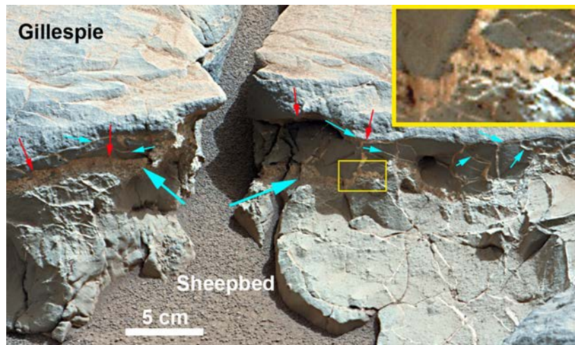
Fig. 30. Image of the contact (marked with red arrows) between the Sheepbed mudstone and the Gillespie Lake sandstone. Illuminated by sunlight from the right, this is a portion of Mastcam Right image 0153MR0008490000201265C00, acquired on Sol 153. Note that the mudstone below the contact shows abundant opening-mode veins with white fill, and that there are abundant subhorizontal veins (turquoise arrows) as well. In a 2 to 3 cm thick horizontal zone beneath the contact (large turquoise arrows), the white fill dominates and contains angular fragments of mudstone (see inset in upper right, enlarged 4 \times ).
