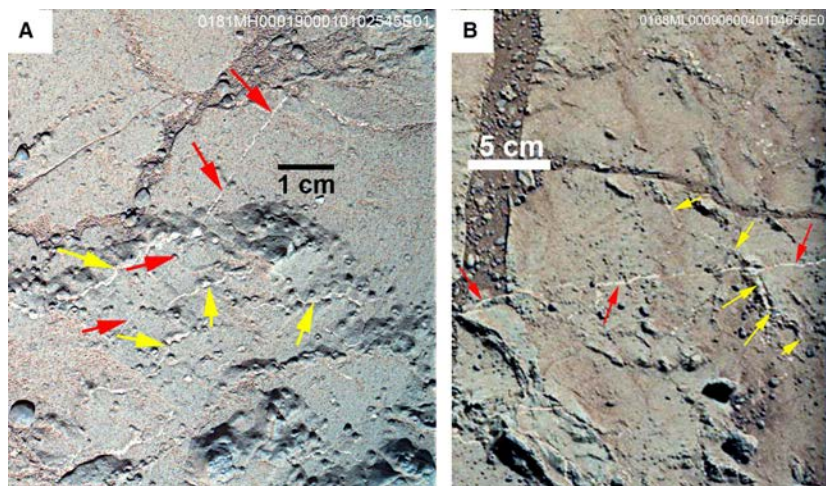
Fig. 28. (A) MAHLI view of a bedding plane with veins (MAHLI image 0181MH0001900010102545E01). Small knobby veins are marked with yellow arrows, straight vein is marked with red arrows and cuts across a knobby vein. (B) Bedding plane view (Mastcam Left image 0168ML0009060040104659E01) with knobby vein (yellow arrows) cut by straight vein (red arrows). MAHLI, Mars Hand Lens Imager.
