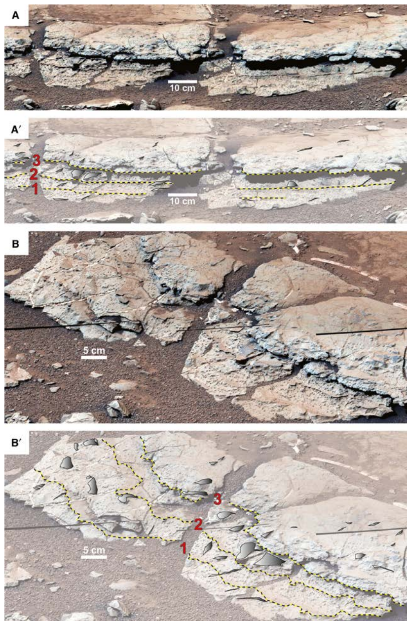
Fig. 6. Prominent layering in the lower portion of Sheepbed unit 2. This interval is more weathering resistant due to diagenetic cements (matrix cement and millimetre-sized nodules) and forms a ‘step’ as the outcrop slopes gently between Sheepbed unit 1 and the Sheepbed/Gillespie contact (Fig. 2B). In both (A) and (B) three thin resistant layers, a few millimetres in thickness, have been sculpted out by aeolian abrasion. These layers are traced with dashed yellow-black lines in images A’ and B’. This interval also shows multiple ‘raised ridges’ (marked as polygons with grey scale gradient in A’ and B’), interpreted as mineralized synaeresis cracks (Grotzinger et al. , 2014; Siebach et al. , 2014). In places, ‘raised ridges’ cut across resistant layers 1, 2 and 3. Note that the upper surface of this more ragged looking interval is comparatively smooth and flat, except where ornamented with ‘raised ridges’: (A) is a portion of a Mastcam Right mosaic acquired on Sol 297 (mcam01238), images 0297MR0012380120203571E01 and 0297MR0012380170203576E01; (B) is a Mastcam Right mosaic acquired on Sol 298 (mcam01246), images 0298MR0012460000203669E01, 0298MR0012460010203670E01, 0298MR0012460020203671E01, 0298MR0012460030203672E01, 0298MR0012460040203673E01 and 0298MR0012460050203674E01.
