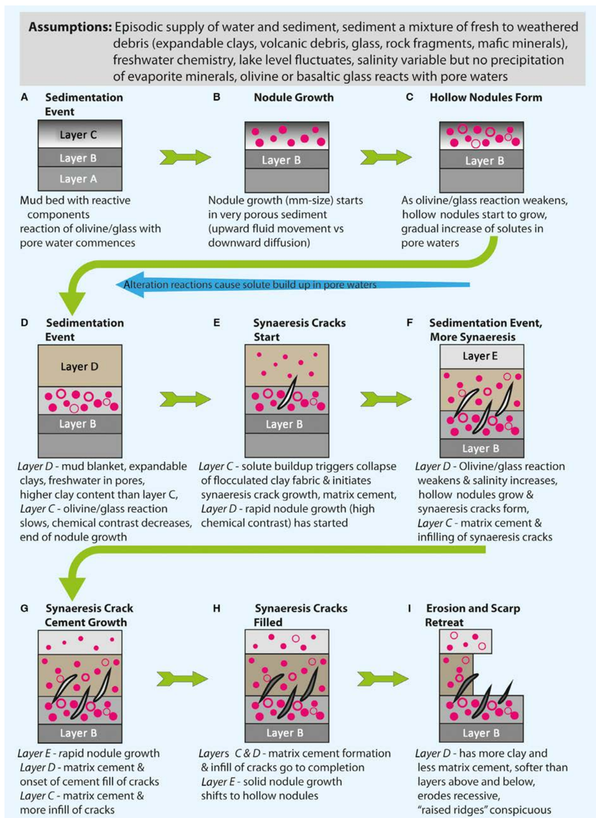
Fig. 21. A summary of how the interplay of sedimentation pulses, diagenetic processes and subsequent erosion produced the features observed in outcrop at Yellowknife Bay.
