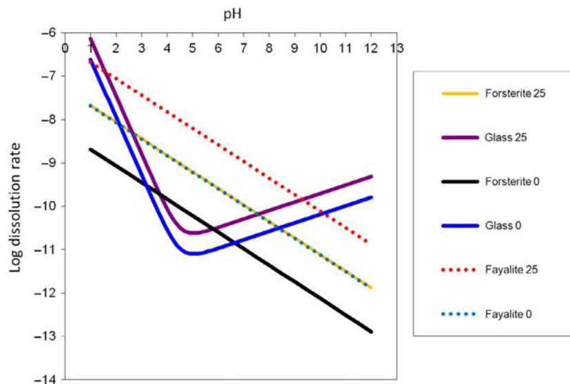
Fig. 10. Dissolution rate laws for fayalite, forsterite and basalt glass at 25°C and 0°C. From Bandstra & Brantley (2008), based on dissolution rates for olivine (Brady & Walther, 1989; Oelkers, 2001a; Pokrovsky & Schott, 2000; Rosso & Rimstidt, 2000; Wogelius & Walther, 1992), basalt (Gislason & Eugster, 1987) and published activation energies for olivine (Van Herk et al. , 1989; Wogelius & Walther, 1992; Jonckbloedt, 1998; Rosso & Rimstidt, 2000; Oelkers, 2001a,b) and basaltic glass (Gislason & Eugster, 1987; Gislason & Oelkers, 2003; Wolff-Boenisch et al. , 2004). The fayalite rate in Fig. 10 is estimated assuming that fayalite dissolves 10 times faster than forsterite (Bandstra & Brantley, 2008) as documented in the literature at acidic to neutral pH (Wogelius & Walther, 1992). Results indicate similar dissolution rates at near neutral conditions for each mineral, suggesting that extensive loss of basaltic glass would probably accompany extensive loss of olivine. However, Martian glass compositions may vary from basaltic glass composition. Proposed chemical compositions for the Mars amorphous material have much lower silica concentrations than basaltic glass (Dehouck et al. , 2014; Vaniman et al. , 2014) with enrichments of Ca and Mg, greatly destabilizing the glass, and higher concentrations of Al and Fe somewhat destabilizing the glass (Oelkers, 2001b). Therefore, the amorphous material on Mars would probably have a dissolution rate higher than the basaltic glass indicated here, indicating that even faster dissolution rates are likely.
