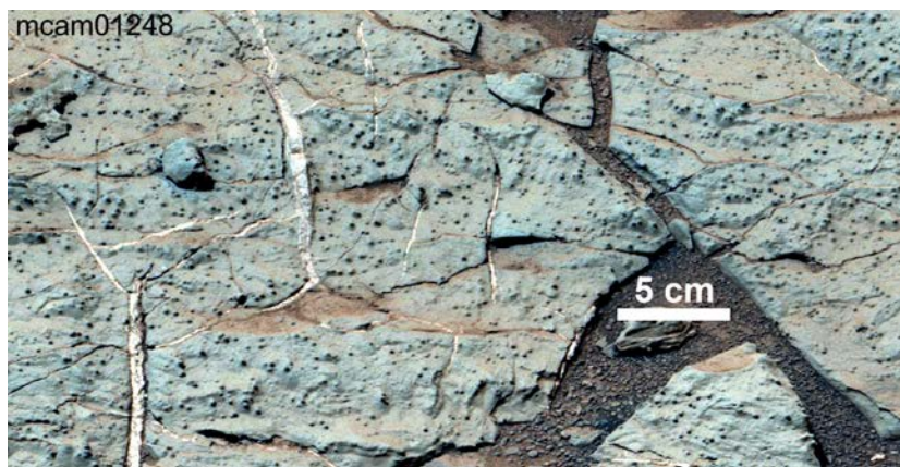
Fig. 12. View of a mudstone bed with abundant small nodules that are sculpted out by aeolian abrasion. The rock is criss-crossed by millimetre to centimetre wide late diagenetic fractures (Grotzinger et al. , 2014) that are filled with calcium sulphate (probably anhydrite; Vaniman et al. , 2014). Given that the rock surface is more or less flush with the anhydrite vein fills suggests that the mudstone is approximately of the same hardness as anhydrite. Images from a Mastcam Right mosaic acquired on Sol 298 (0298MR0012480180203696E01, 0298MR0012480230203701E0, 0298MR0012480240203702E01 and 0298MR0012480290203707E01).
