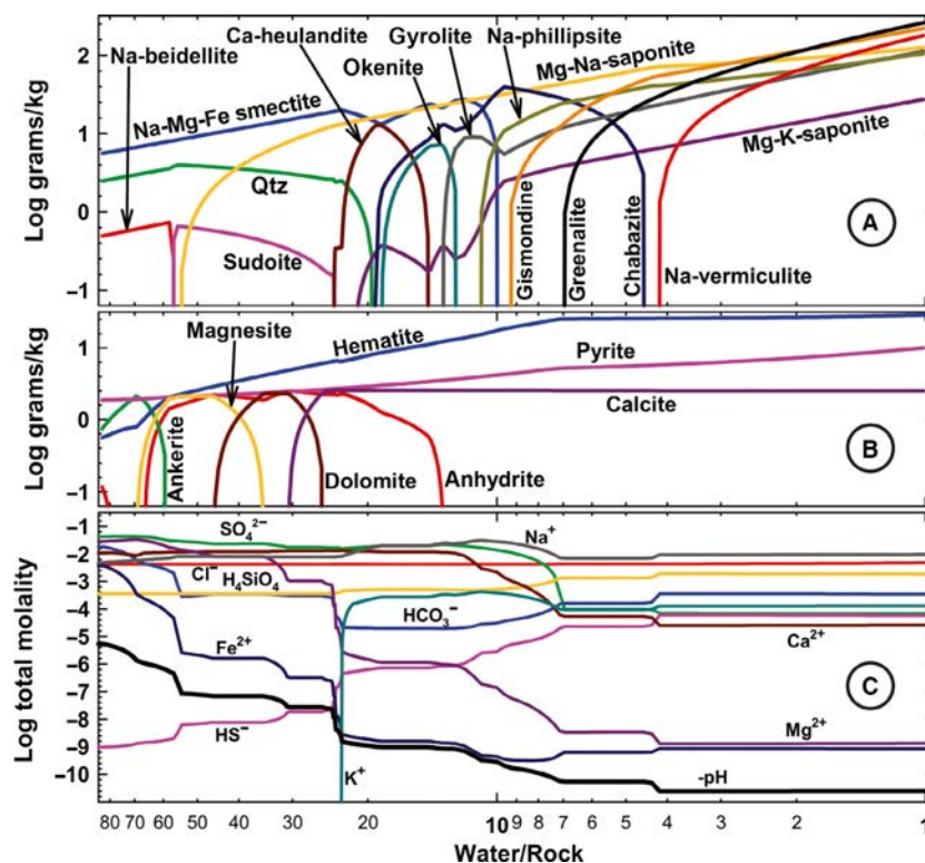
Fig. 11. Computed reaction of Mazatzal basalt with a hypothetical Sheepbed runoff/basin fluid described in the text. (A) and (B) Logarithm of mass of precipitated minerals per kilogram of initial aqueous phase versus water/rock ratio (mass ratio of titrated basalt to original aqueous phase mass). The logarithmic scale makes it difficult to compare masses visually, for example, at w/r 15, calcite mass is 2.5 g, Mg-Na-saponite is 20.6 g and Na-Mg-Fe smectite is 22.1 g. (C) Composition of the aqueous phase in total molality of component species (not individual species). The steps and plateaus in pH and dissolved component concentrations reflect buffering by the various mineral assemblages. At any given w/r, the graphs show the thermodynamically stable mineral assemblage and aqueous composition for the particular bulk composition specified by the w/r. The graph does not portray an amount of as yet unreacted detrital basalt material that is intermingled with the computed authigenic minerals; the unreacted material dilutes the authigenic assemblage to an extent dependent on a sedimentological conception of the reacting environment.
