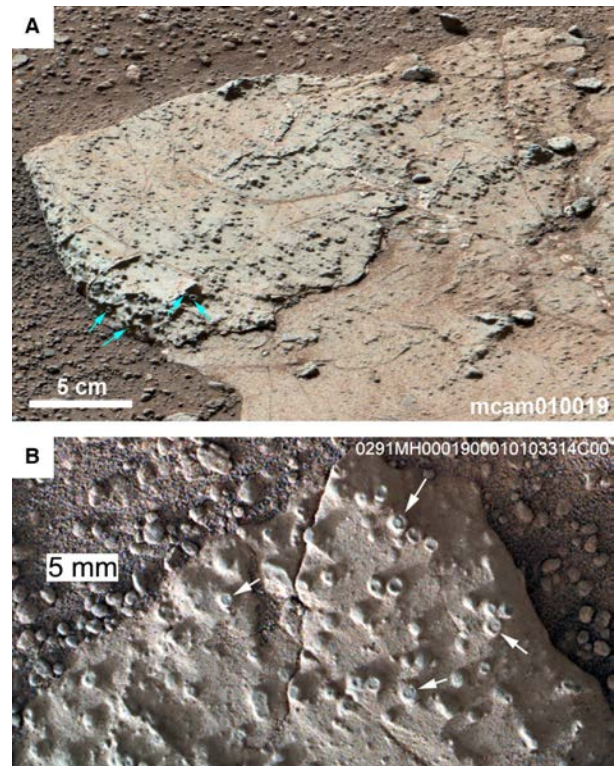
Fig. 19. (A) Weathering resistant bed with abundant solid as well as hollow nodules. Arrows point to hollow nodules whose openings point sideways, possibly nodules that were cored with an earlier and more soluble (or softer) material that was removed by dissolution or abrasion once the protective outer shell of the nodule was breached. Portion of Mastcam Right mosaic acquired on Sol 192 (images 0192MR0010190170202632E01 and 0192MR0010190180202633E01). (B) A resistant slab of sediment covered with 'hollow nodules'. Many of these, however, contain a soft greenish fill (arrows) that is at various stages of being removed, probably by aeolian erosion that selectively removes the soft fills. MAHLI image 0291MH0001900010103314C00. MAHLI, Mars Hand Lens Imager.
