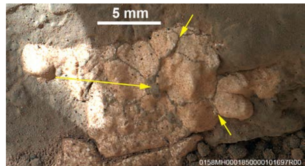
Fig. 27. A look at a fracture surface with anhydrite stuck to the wall. The anhydrite consists of impinging-coalescing spherules that have thin films (short arrows) and pockets (long arrow) of grey matrix material between them. From MAHLI image 0158MH0001850000101697R00. MAHLI, Mars Hand Lens Imager.
