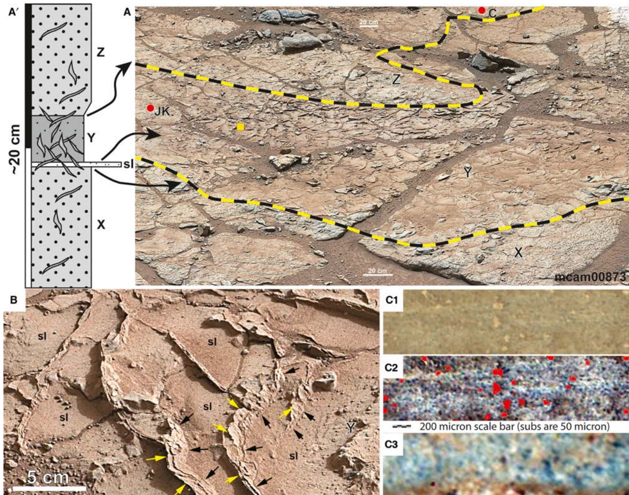
Fig. 7. (A) and (A') Small-scale stratigraphic relationships at the John Klein locality. The outcrop slope and bed attitude suggest that below the ridge-bearing interval (layer Y), there is a mudstone with millimetre-sized nodules (layer X), and that the ridge-bearing layer is overlain by another mudstone (layer Z) with millimetre-sized nodules. Approximate boundaries are drawn as yellow-black dashed lines. Red circles mark the John Klein and Cumberland drill sites: (A) is a Mastcam Left mosaic acquired on Sol 162 (mcam), images 0298MR0012460000203669E01, 0298MR0012460010203670E01, 0298MR0012460020203671E01, 0298MR0012460030203672E01, 0298MR0012460040203673E01 and 0298MR0012460050203674E01. (B) A closer view of the ridge-bearing surface shows a basal planar layer (sl; presumed sandy) that is cross-cut by 'raised ridges'. Ridges can be either vertical or cut through obliquely (yellow arrows). Black arrows mark the break between the basal sandy layer (sl) and the ridges. Some of the vertical ridges show symmetrical internal layering, probably isopachous cements. At right there is sediment of layer Y that is still being eroded. Elsewhere erosion has 'cleaned off' the softer material, of layer Y, and exposed the surface of the resistant sandy layer. Mastcam Right images 0164MR0008850100201599E01 and 0164MR0008850110201600E01. (C) Comparison of grain size in basal layer (sl) with grain size typical for Sheepbed mudstone. (C1) MAHLI image from Ekwir brush spot (Sol 150, 0150MH0001690010101421C00), brownish-beige spots are surficial sand grains; (C2) enhanced version of C1 (aeolian dust marked in red). (C3) MAHLI close-up of resistant basal layer (sl) that appears definitely coarser and has grains in the very fine to fine sand size range (0165MH0001880010101995C00). MAHLI, Mars Hand Lens Imager.
