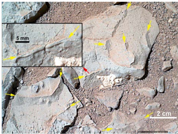
Fig. 18. Blocks of erosion-resistant nodule-bearing mudstone. Linear features marked with yellow arrows are interpreted as 'raised ridges' that are buried in a well-cemented matrix. Inset shows close-up of one of these ridges (red arrow). The ridge appears to have symmetrical cementation with harder margins and a softer interior, just as described from raised ridges in softer strata. The material that fills the 'ridge' does not appear to be significantly different from the surrounding matrix and implies that the cementing agent in the fracture and the surrounding matrix is probably the same. MAHLI image 0158MH0000750010101569C00. MAHLI, Mars Hand Lens Imager.
