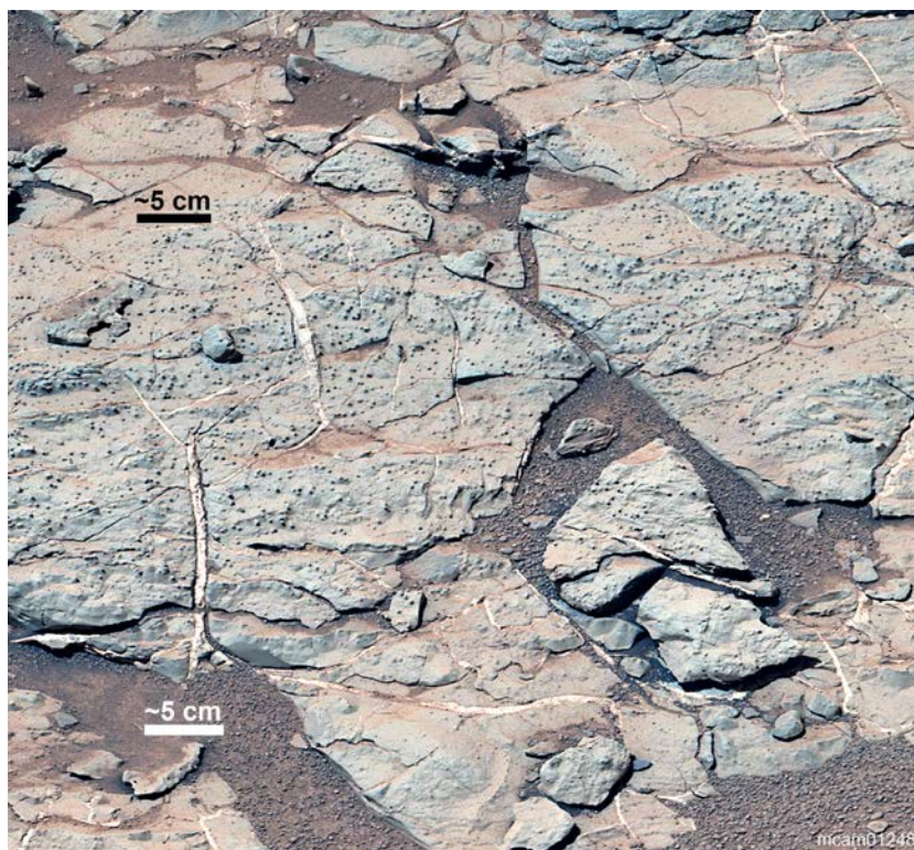
Fig. 22. Oblique view of the Sheepbed outcrop with a nodule-rich bed in the middle-ground. Parallel-sided anhydrite-filled subvertical fractures (up to 1 cm wide) are prominent. These ‘straight veins’ represent one of the common styles of vein formation in the Yellowknife Bay area (Fig. 2). Strike of veins appears to be random, consistent with a hydrostatic state of stress in the plane of bedding during their formation. The veins weather level with their mudstone host indicating that the two have approximately the same resistance to aeolian abrasion. Portion of a Mastcam Right image from Sol 298 (images 0298MR0012480180203696E01, 0298MR0012480230203701E01, 0298MR0012480240203702E01 and 0298MR0012480290203707E01).
