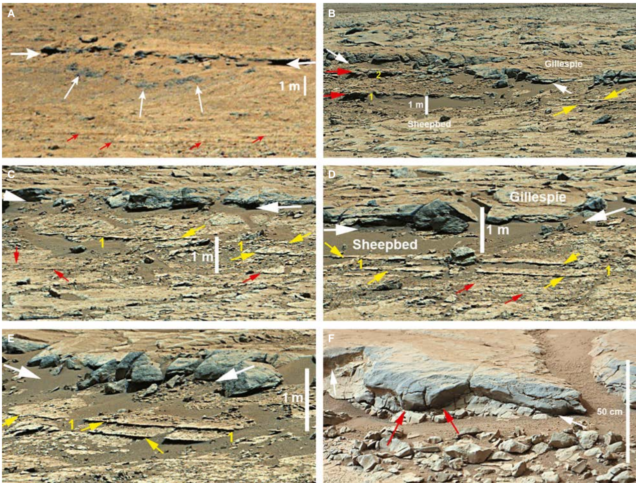
Fig. 3. Details from panoramas (B) and (C) in Fig. 2. The lettering of images corresponds to white lettering used in Fig. 2. All distances refer to distance between Sol 137 location (Fig. 2) and escarpment that marks the Sheepbed/Gillespie contact in a given image. (A) Distal (164 m NE of Sol 137 location) view of escarpment that shows the Sheepbed/Gillespie contact (marked with white arrows in this and following images), and a more resistant rock body with a concave base (small arrows) within the Sheepbed unit. Mastcam Right images 0137ML0008180250104170E01 and 0137ML0008180000104145E01. (B) Well-developed bedding in the Sheepbed mudstone (75 m distance). At left two thick resistant beds ( ca 15 cm thick, levels 1 and 2, red arrows), probably sandstones based on their weathering resistance. They show internal stratification and appear to thin towards the right. The upper bed, marked 2, is truncated at the Sheepbed/Gillespie contact (white arrows), the lower one, marked 1, seems to pass into a thinner and less resistant bed to the right (upper yellow arrow). The lower yellow arrow points to a similar bed that appears to be covered to the left. At this location, the truncation surface cuts down about 50 cm into the Sheepbed mudstone. Mastcam Right images 0147MR0008340000201175E01 and 0147MR0008340010201176E02. (C) About 61 m distant, the level 1 couplet of resistant beds (yellow arrows) from previous image, and additional resistant beds below them (red arrows). Mastcam Right images 0147MR0008340020201177E01 and 0147MR0008340030201178E01. (D) The same couplet (yellow arrows) at ca 51 m distance, as well as stratigraphically lower positioned resistant beds (red arrows). Mastcam Right image 0147MR0008340040201179E01. (E) Continuation of level 1 couplet at ca 41 m distance. Mastcam Right 0147MR0008340060201181E01. (F) The base of the Gillespie sandstone with a deep scour (red arrows) into the Sheepbed mudstone. The scour surface shows up to 25 cm relief. Mastcam Right image 0137MR0008170280200961E01.
