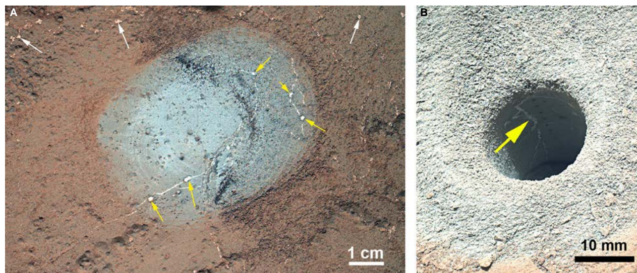
Fig. 23. (A) An area brushed with the DRT (Fig. 1) at the end of the rover arm. Note the colour difference between brushed and un-brushed surface. Rounded bodies of likely anhydrite occur across the surface and are comparatively easy to see (white arrows). The dust obscures the fact that these are connected to anhydrite-filled fractures, but that relationship is readily observed in brushed areas (yellow arrows). The anhydrite lumps are irregular in shape and size. MAHLI image 0173MH0001900010102313C00. (B) MAHLI image of the interior of the John Klein drill hole, showing the contrast between the unoxidized rock on the interior and the brownish oxidized coating at the surface. The yellow arrow points to an anhydrite vein that is oriented subvertical and has subhorizontal offshoots. MAHLI image 0270MH0002520000102916R00. MAHLI, Mars Hand Lens Imager.
