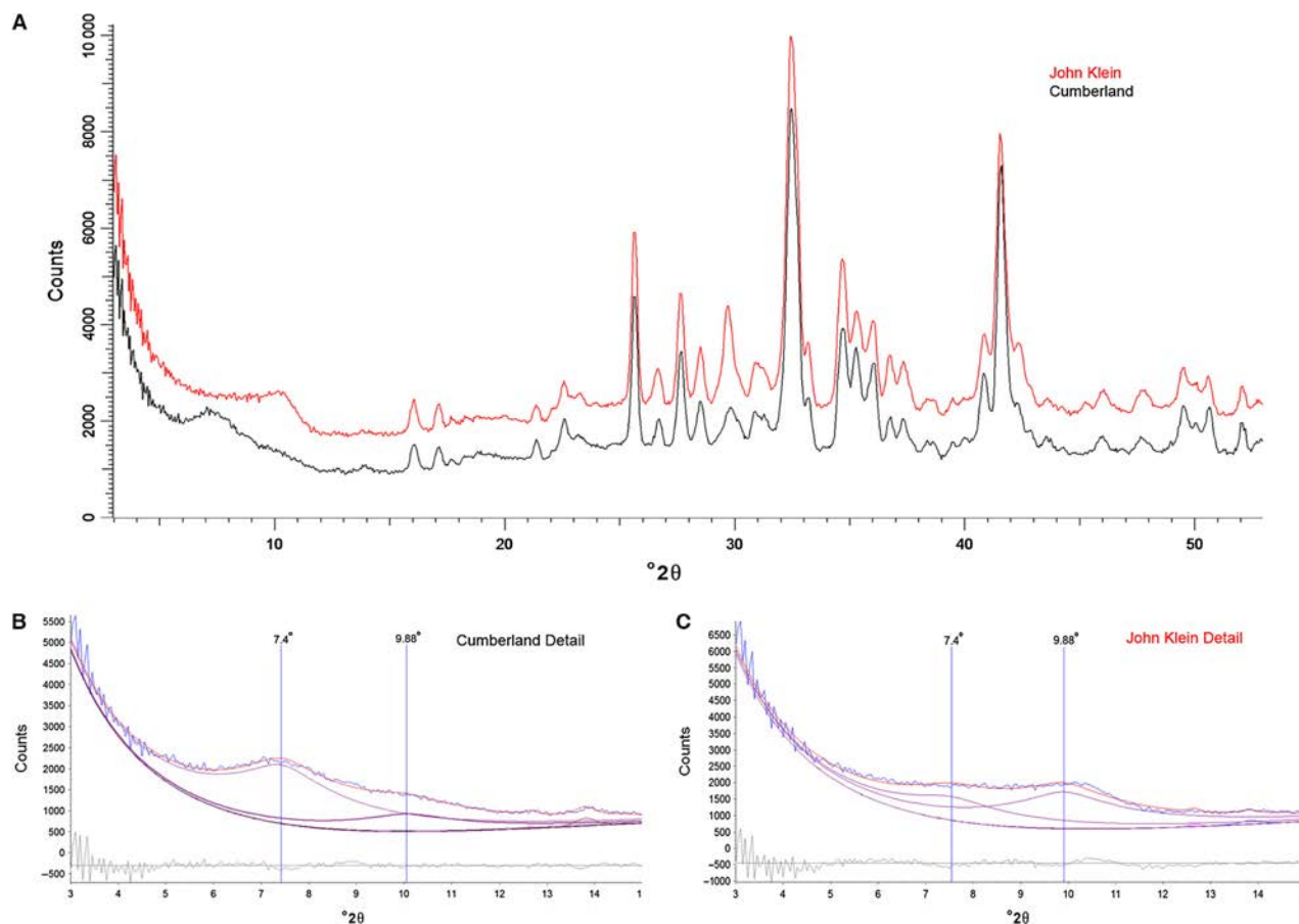
Fig. 9. (A) X-ray diffraction patterns of the two drill samples collected from the Sheepbed mudstone. The complete diffraction patterns illustrate how similar both samples are, with the exception of the clay mineral diffraction features at low angles. (B) and (C) Show the expanded low-angle portion of these patterns and illustrate the distinct difference in clay minerals between the two samples, with a pronounced broad 14 Å feature (with a lesser 10 Å feature) in the Cumberland samples and a pronounced 10 Å feature (with a smaller 14 Å feature) in the John Klein sample. Note scattering at small diffraction angles, a potential indication of a short-range ordered material such as Fe-allophane, a clay mineral precursor phase.
