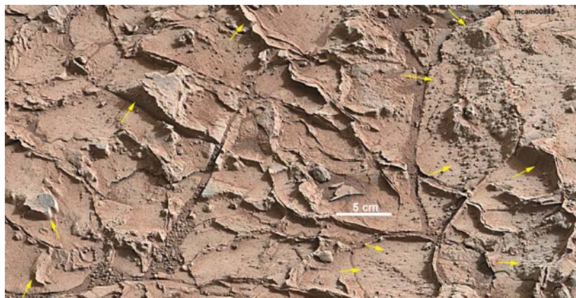
Fig. 16. Close-up of raised ridge horizon (layer Y) at John Klein drill location. Shows that erosion-resistant ridges protected matrix material in various places (arrows) from complete erosion. This matrix contains nodules and there are wind tails associated with nodules, suggesting a softer material, similar to elsewhere in layer Y (for example, Fig. 15D). Towards the upper right corner the ridges appear to get ‘buried’ under more resistant material with nodules, probably the transition to the overlying layer Z (Figs 13 and 15). Portion of a Mastcam Right mosaic acquired on Sol 164 (images 0164MR0008850020201591E01, 0164MR0008850050201594E01, 0164MR0008850060201595E01 and 0164MR0008850070201596E01.)
