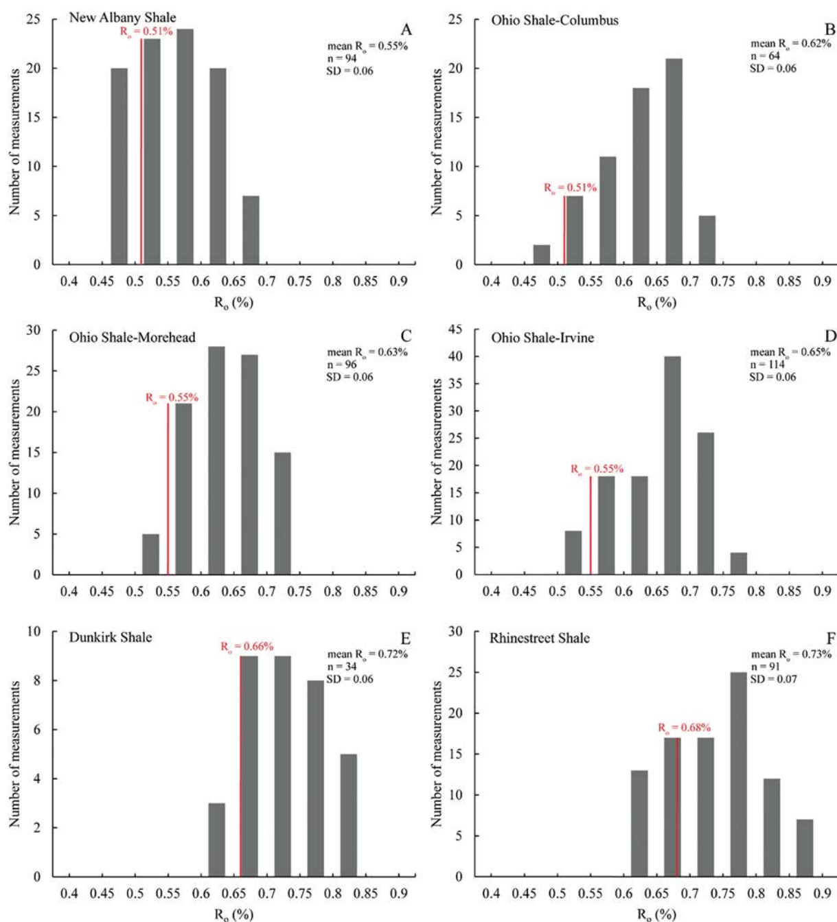
Fig. 10. Histograms of measured R_o of dispersed vitrinite particles in shales that enclose coal lenses. (A) New Albany Shale from Shepherdsville, KY; (B) Ohio Shale from Columbus, OH; (C) Ohio Shale from Morehead, KY; (D) Ohio Shale from Irvine, KY; (E) Dunkirk Shale from Dunkirk, NY; (F) Rhinestreet Shale from Derby, NY (Table 1). n = number of measurements; SD = standard deviation. Red bar indicates the mean R_o of enclosed coals. (For interpretation of the references to colour in this figure legend, the reader is referred to the web version of this article.)
