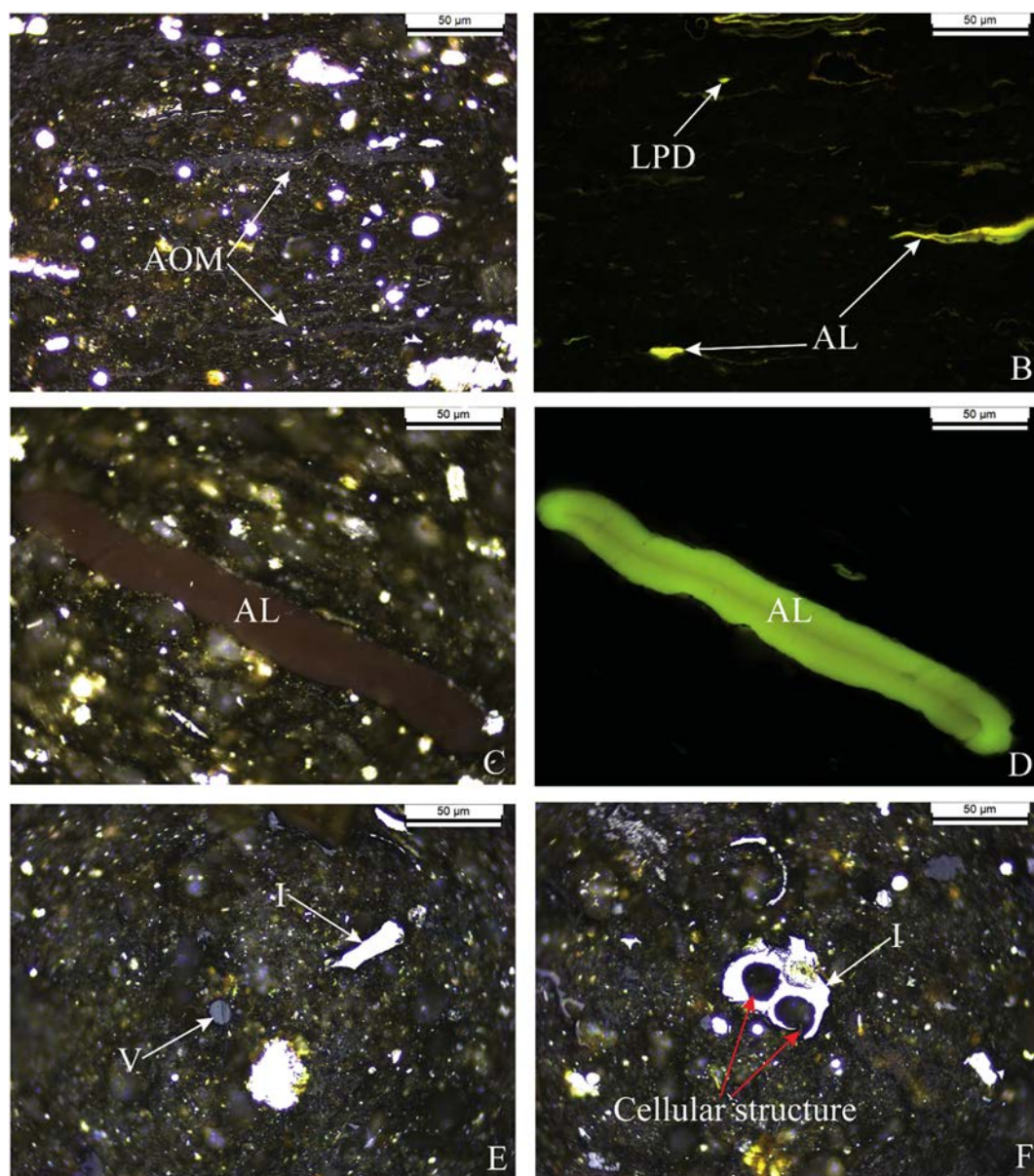
Fig. 5. Photomicrographs of primary macerals in black shales in reflected white light and oil immersion (A, C, E, F) and in fluorescence mode (B, D). Panels B and D show the same field of view as panels A and C in fluorescence mode, respectively. Note that the cellular pores in inertinite in panel F are filled with mineral matter, probably diagenetic silica. New Albany Shale sample from Shepherdsville, KY. AOM = amorphous organic matter; AL = alginite; LPD = liptodetrinite; V = vitrinite; I = inertinite.
