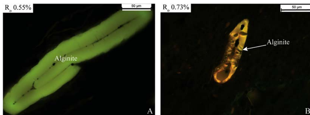
Fig. 7. Photomicrographs of alginite derived from Tasmanites cysts in the New Albany Shale (A) and the Rhinestreet Shale (B) in fluorescence mode.
