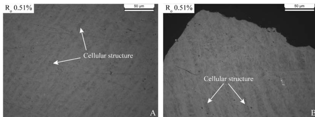
Fig. 4. Photomicrographs of vitrinite with preserved cellular structures in coal samples in reflected white light and oil immersion. Coal sample in the New Albany Shale from Shepherdsville, KY.
