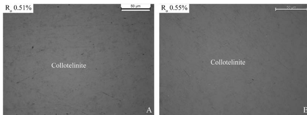
Fig. 3. Photomicrographs of collotelinite in coal samples in reflected white light and oil immersion. (A) Coal sample in New Albany Shale from Shepherdsville, KY. (B) Coal sample in the Ohio Shale from Morehead, KY.
