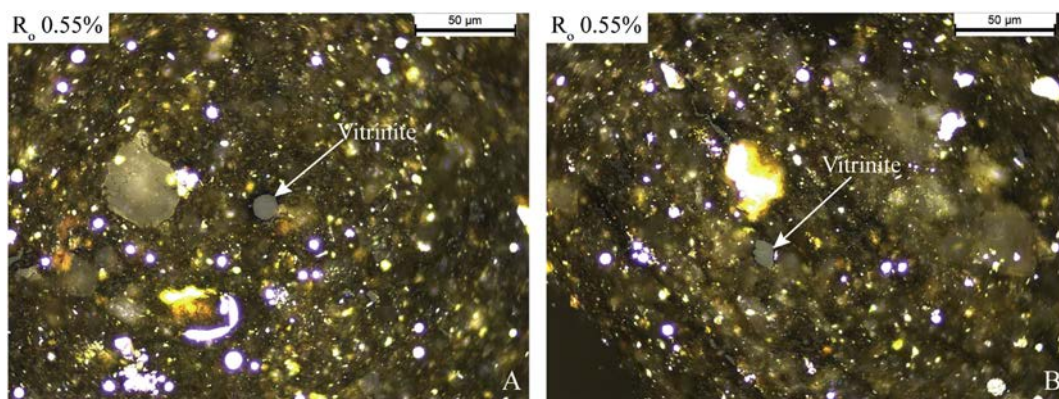
Fig. 13. Photomicrographs of dispersed vitrinite particles in shales in reflected white light and oil immersion. (A) Rounded vitrinite particles that could be cor-pogelinite. (B) Vitrinite particles with sharp edges that could be fragments of collotelinite. New Albany Shale sample from Shepherdsville, KY.
