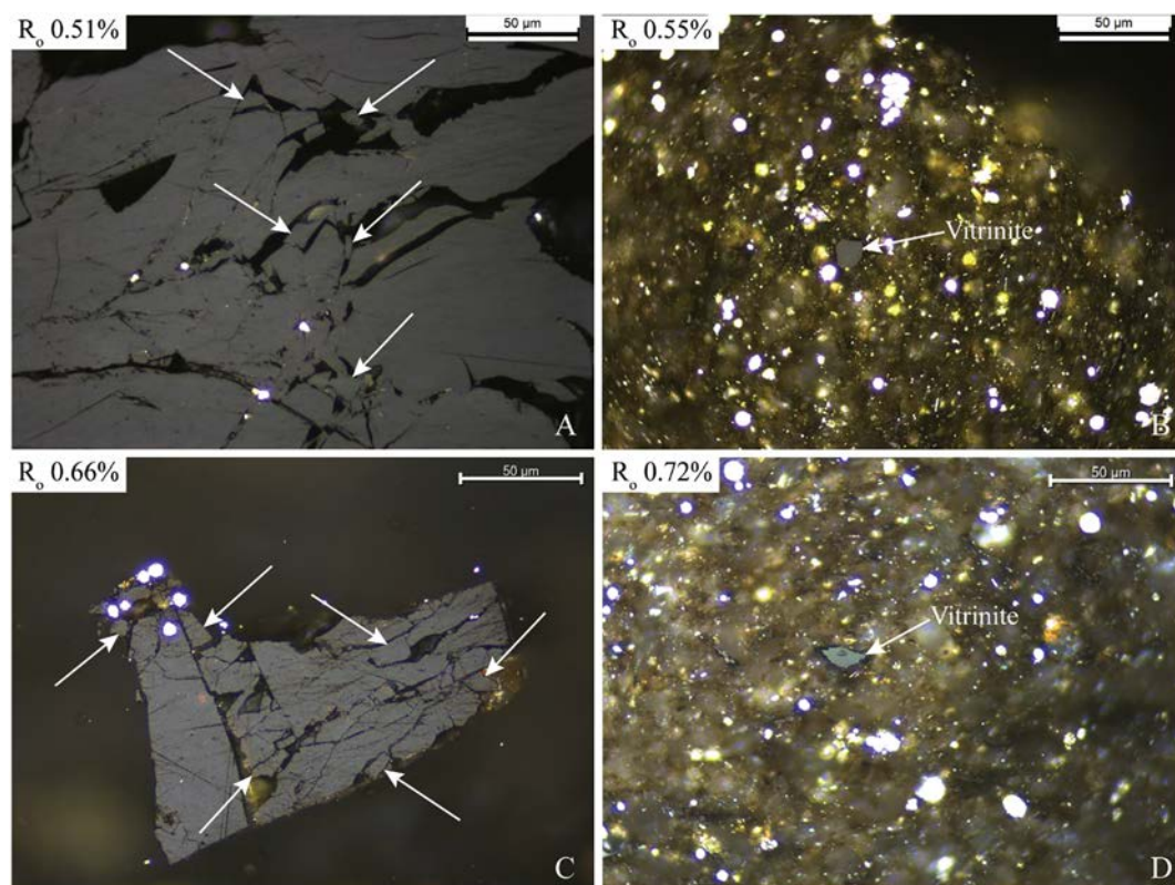
Fig. 6. Photomicrographs of vitrinite fragments (white arrows) in coals (A, C) and dispersed vitrinite particles in shales (B, D) that enclosed the coal samples in reflected white light and oil immersion. (A – B) Coal and shale samples from the New Albany Shale from Shepherdsville, KY. (C – D) Coal and shale samples from the Dunkirk Shale from Dunkirk, NY.
