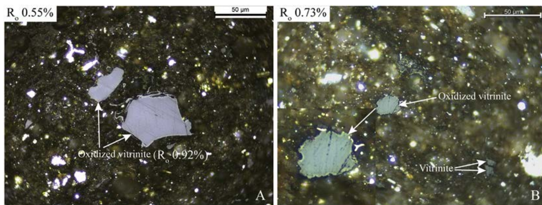
Fig. 11. Photomicrographs of oxidized vitrinite in reflected white light and oil immersion. (A) New Albany Shale from Shepherdsville, KY. Note the sharp edges of the vitrinite particles and the oxidized rim of the larger vitrinite particle. These two particles were excluded for R_o measurements. (B) Rhinestreet Shale from Derby, NY. Insert image is the close-up view of the oxidized vitrinite particle showing an oxidized rim.
