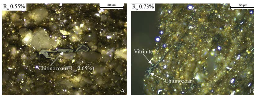
Fig. 12. Photomicrographs of chitinozoan fragments in the New Albany Shale (A) and the Rhinestreet Shale (B) in reflected white light and oil immersion. Note that the vitrinite-like particle next to a chitinozoan fragment in panel B has a comparable reflectance to the chitinozoan fragment, suggesting that it could be a chitinozoan fragment cut perpendicular to the chitinozoan. R_{ch} = chitinozoan reflectance.
