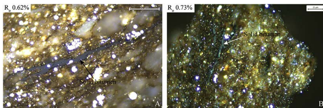
Fig. 8. Photomicrographs of solid bitumen in the Ohio Shale from Columbus (A) and the Rhinestreet Shale (B) in reflected white light and oil immersion.
